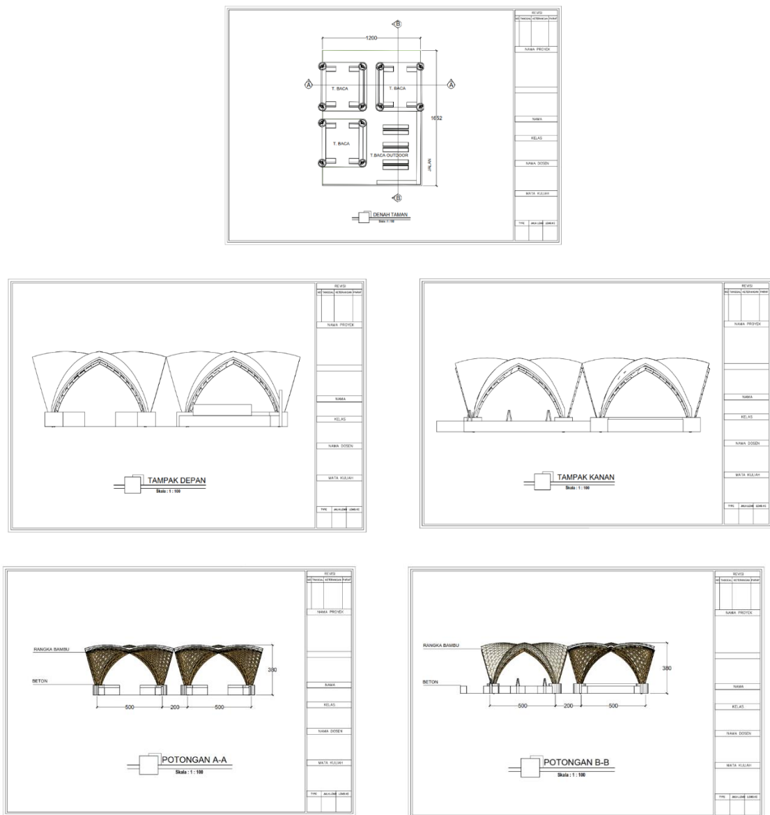
Gambar 5. Gambar Detail Engineering Design (DED) 2D Taman Baca Madrasah Tsanawiyah Pondok Pesantren Wihdatul Ulum
