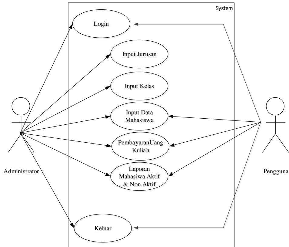
Gambar 3. Usecase Diagram
