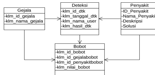
Gambar 2. Class Diagram Sistem Pakar
