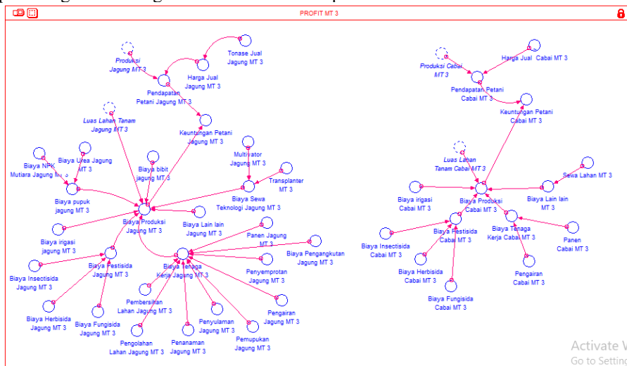
Gambar 6. Sub Model Profit
