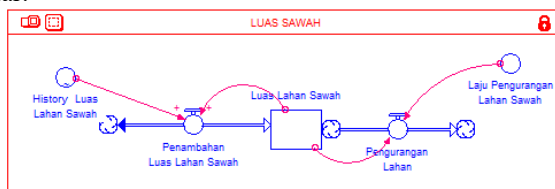
Gambar 4. Stock and Flow Diagram Sub Model Luas Lahan Sawah
